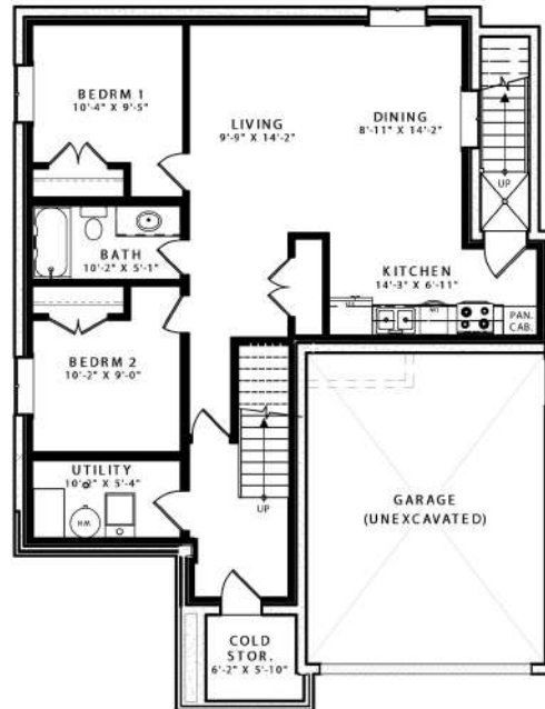
LOWER FLOOR PLAN APARTMENT - 806 sq. ft
