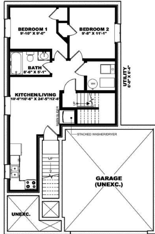
LOWER FLOOR PLAN APARTMENT - 595 sq. ft
