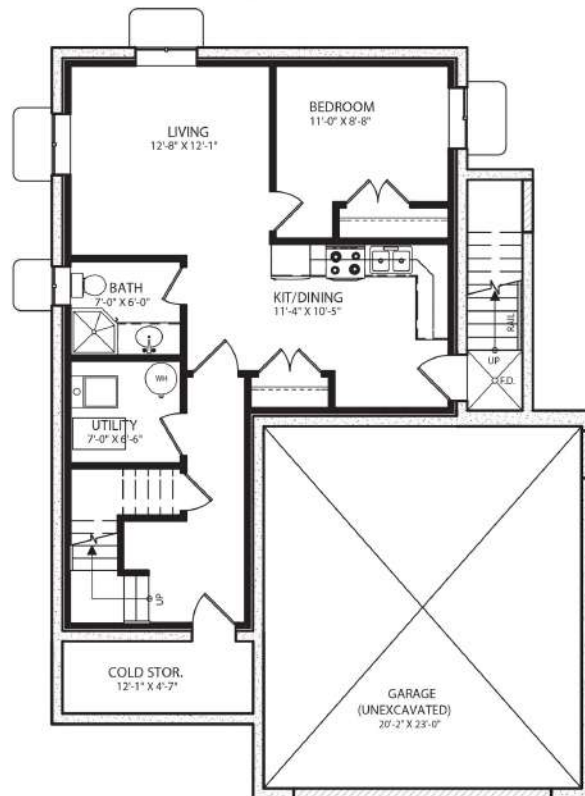
LOWER FLOOR PLAN APARTMENT - 818 sq. ft
